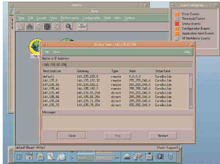
Figure 3. The output of MIB ipRouteTable group retrieved by HP OpenView.
